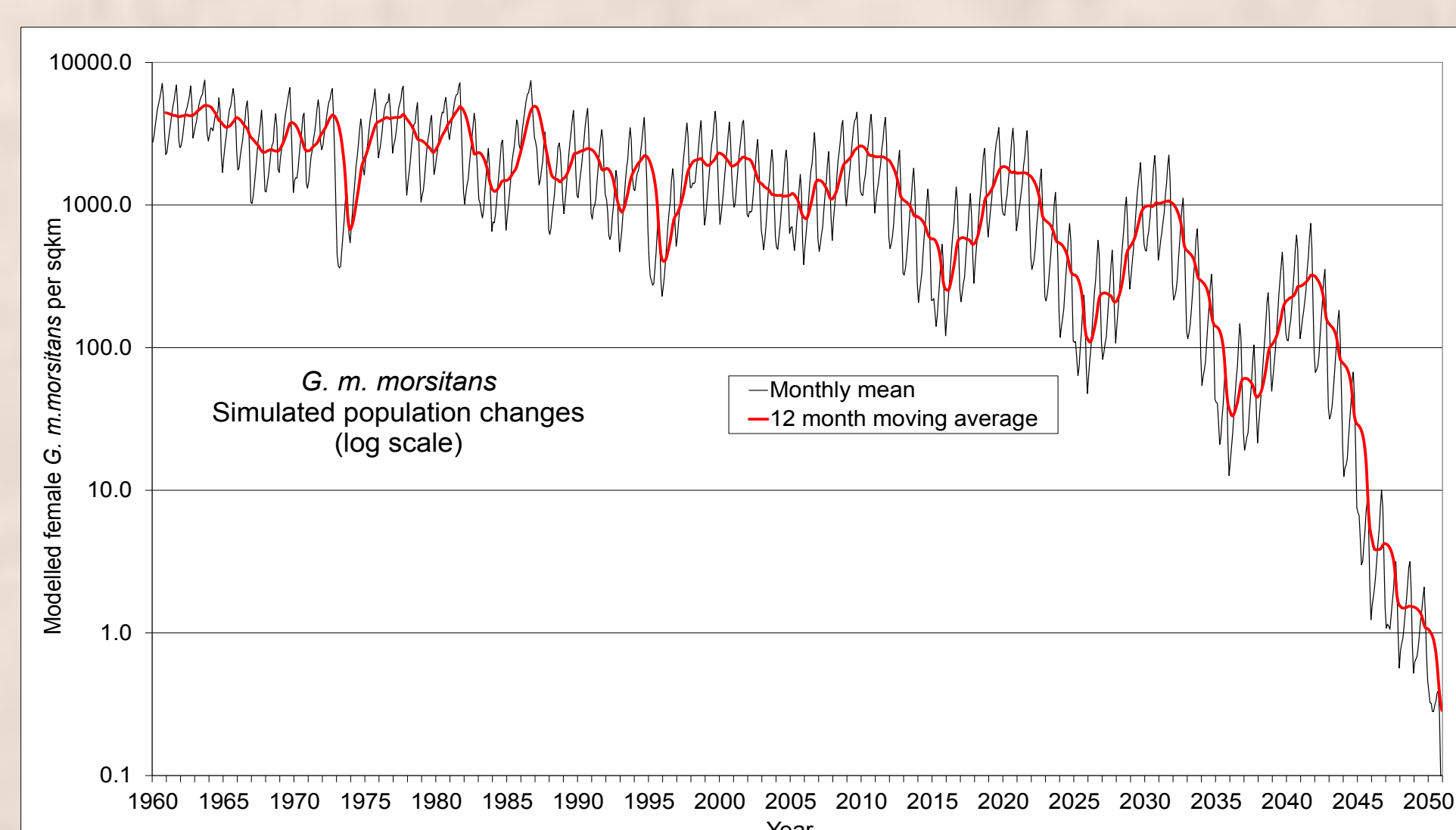
Figure 2: Rekomitjie Research station 1960-2050
